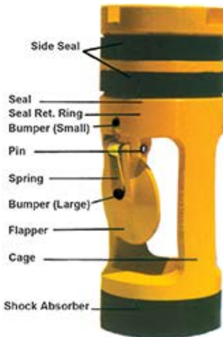
Flapper Type
